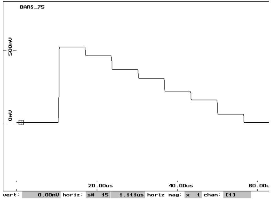
Figure 1-8: 75% Color bars — Y channel
