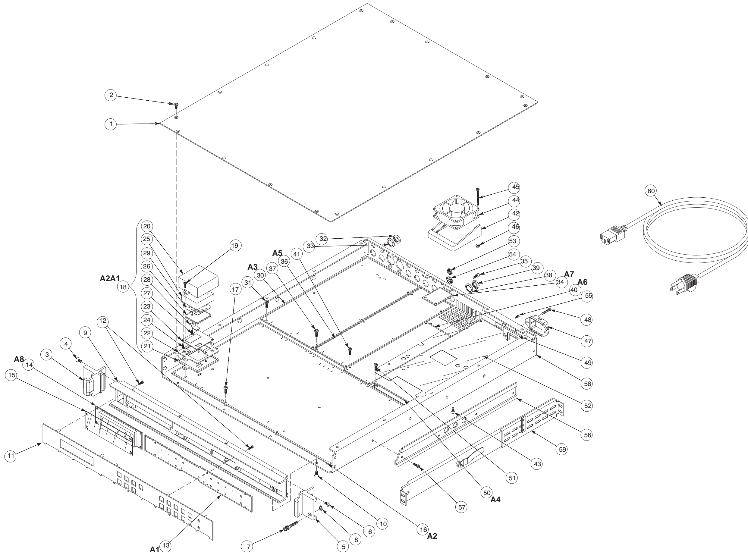
Fig. 1 Exploded view
