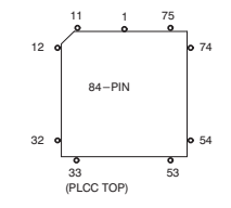
84-PIN PLCC
