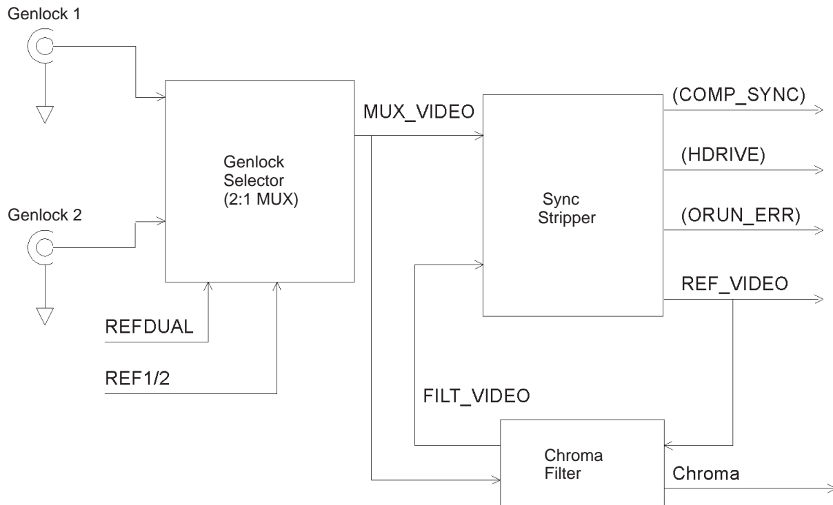
Figure 3-2: Block diagram of genlock Input <1>
